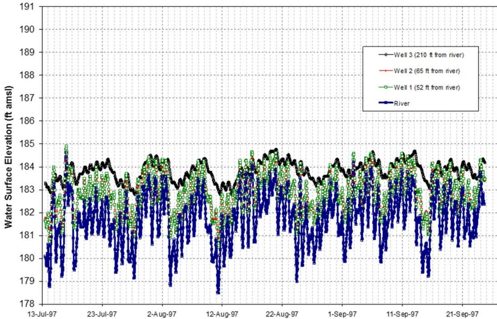
Comparison of Water Surfaces in Monitoring Wells with River Surface
