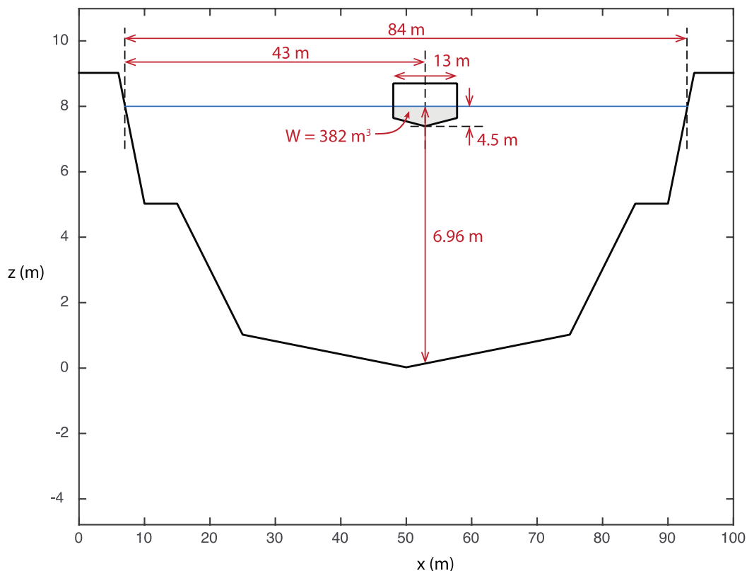
Figure 12. Definition sketch of the example solution.
