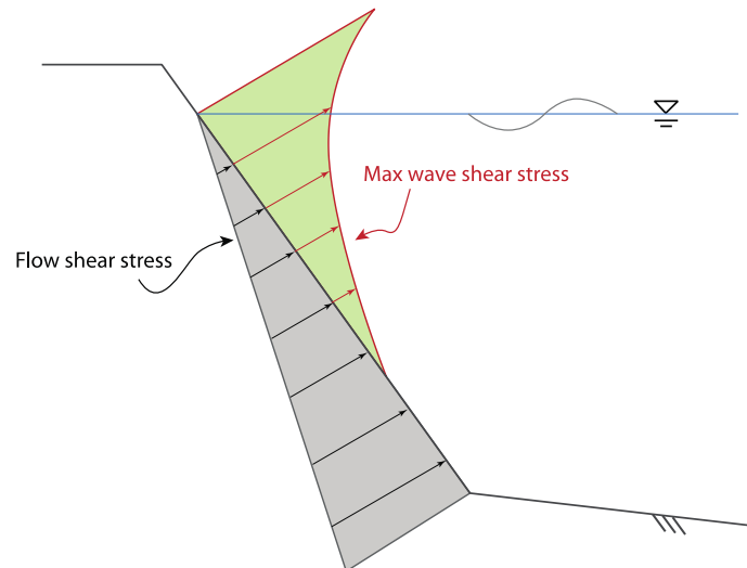
Figure 12. Wave and flow shear stress distributions on the bank.
