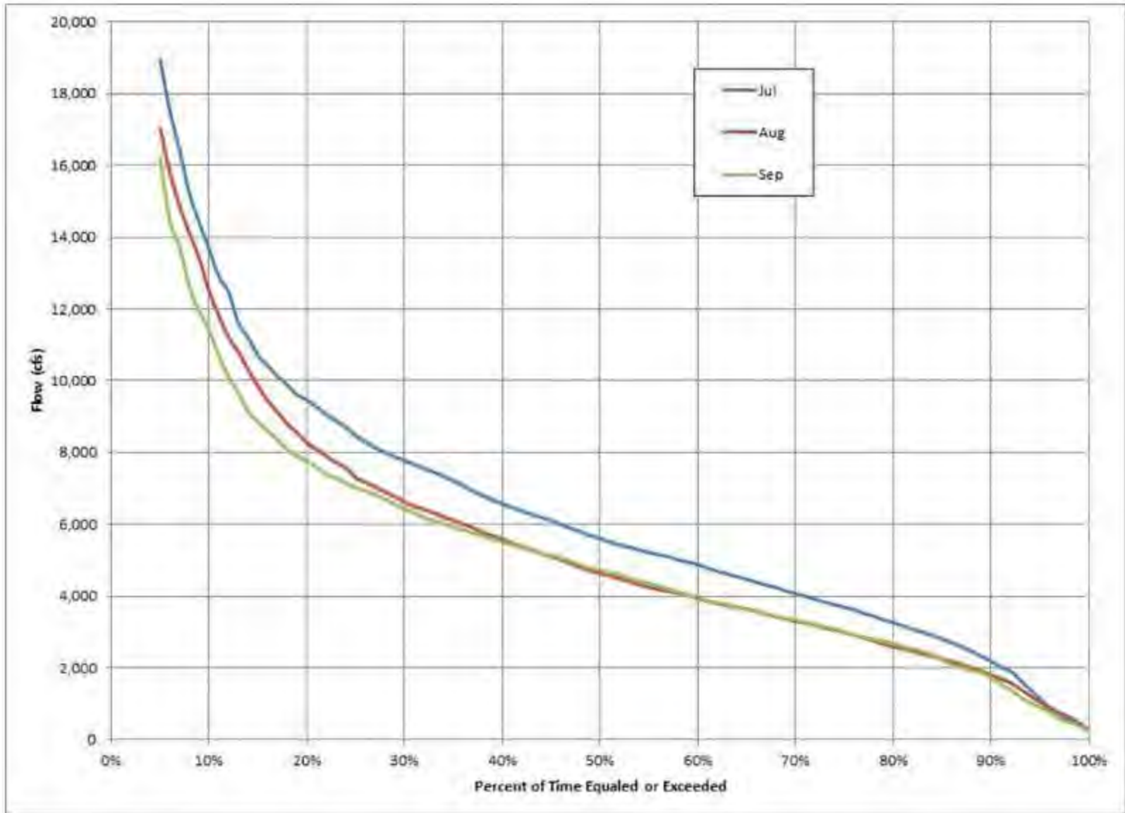
Figure 3.2-4: Connecticut River at Montague USGS Gage- Jul, Aug and Sep Duration Curve (1940- present)
