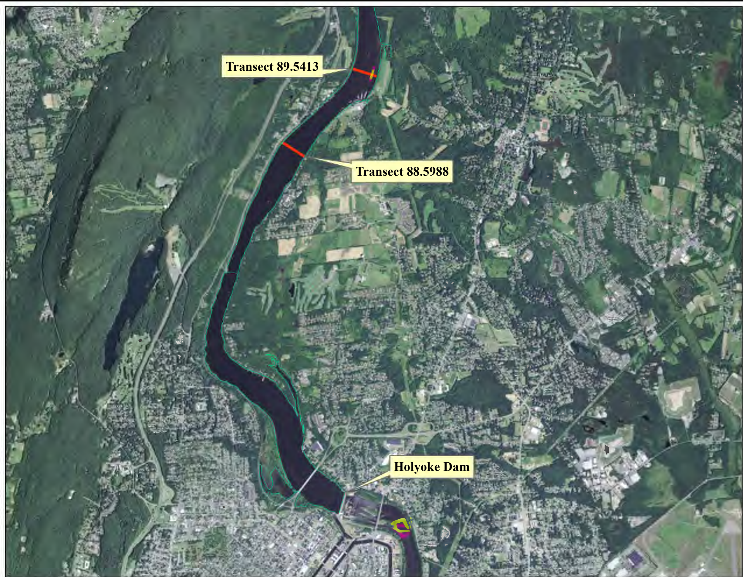
FIRSTLIGHT POWER RESOURCES IFIM Figure 5.3.5-1: Reach 5 HEC-RAS Transects Page 4 of 4
