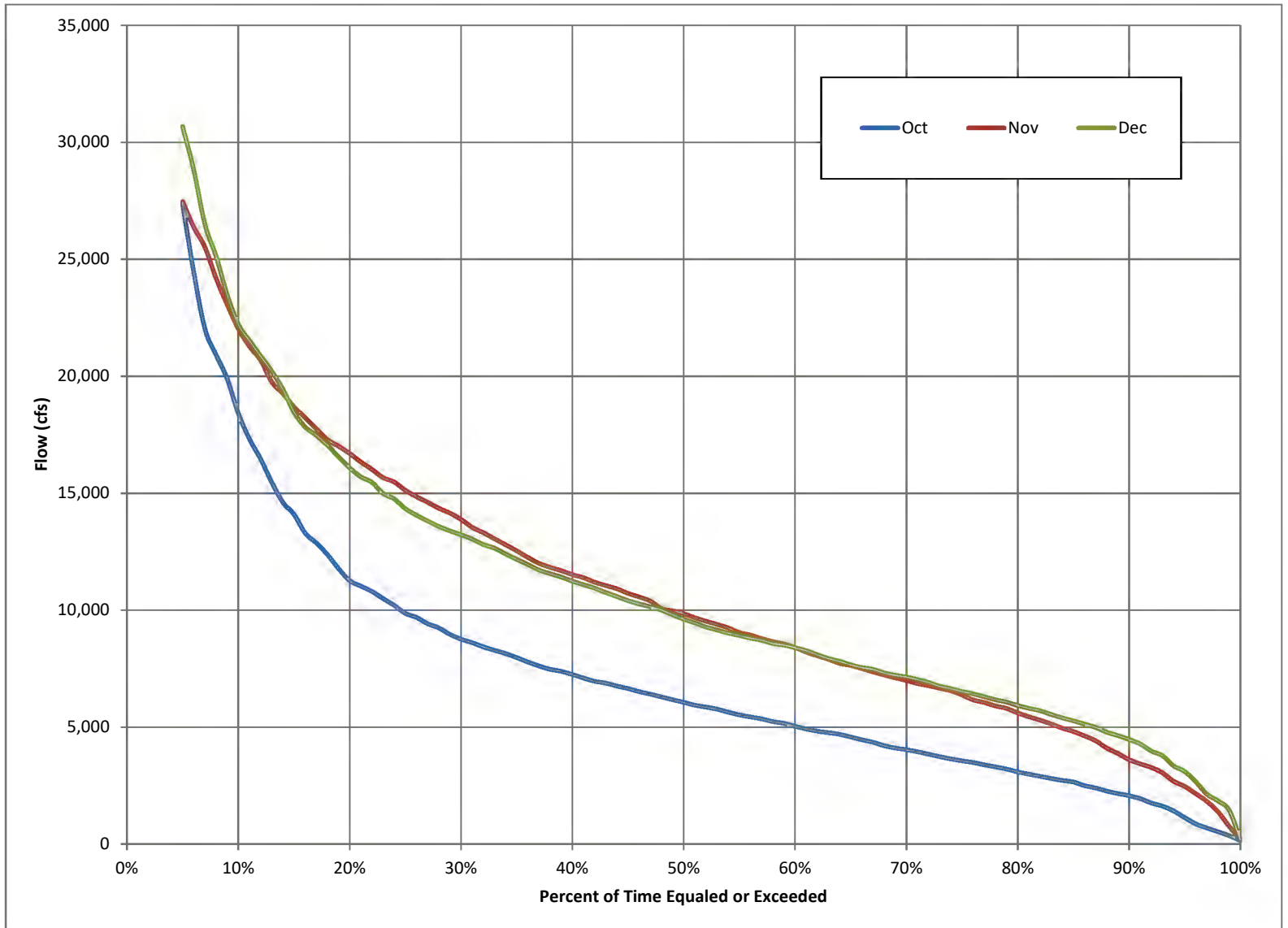
Figure 3.1-5: Connecticut River at Turners Falls Dam- Oct, Nov and Dec Flow Duration Curve (1940- present)
