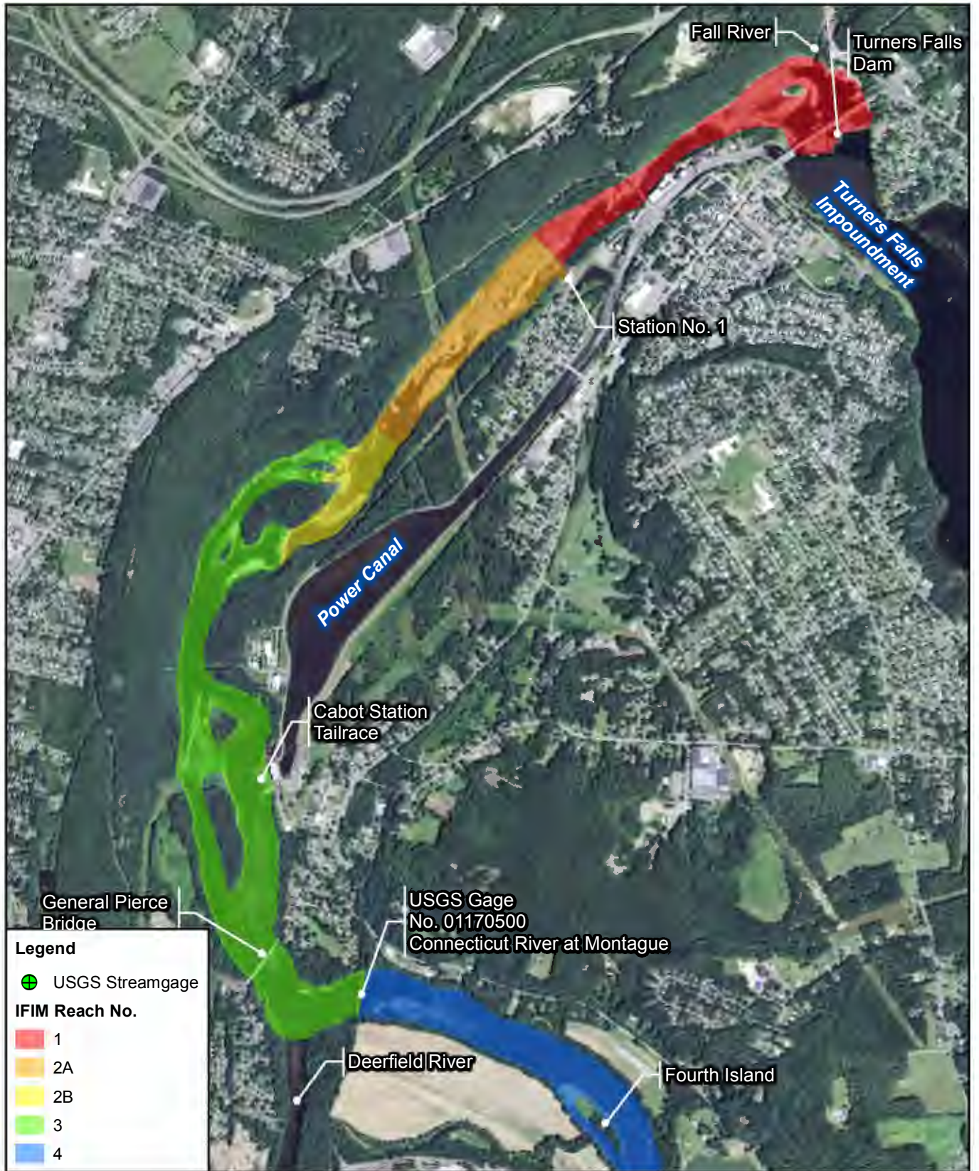
Figure 4.1-2: Instream Flow Study Reaches 1 thru 3 - Bypass Reach
