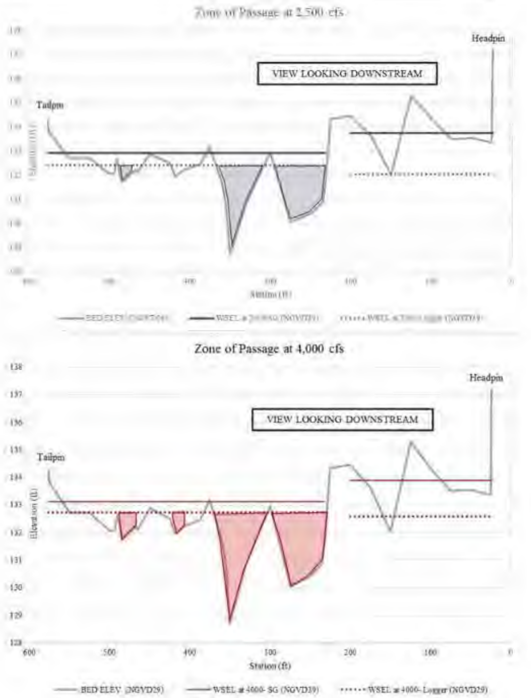
Figure 6.1.1.3-4 (cont): Cross Sectional Area (Shaded) Meeting Body Depth Requirements of American shad at Passage Barrier in Left Channel (Flow values relate to gate releases, not flow in channel)
