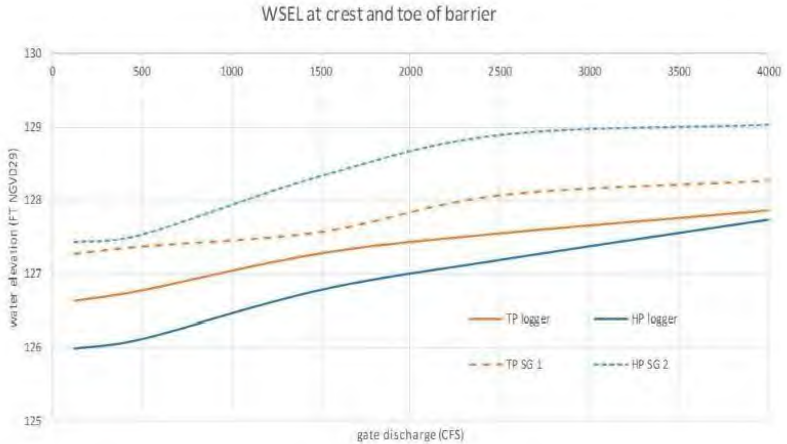
Figure 6.1.1.3-3: Water Elevations at Toe and Crest of Passage Barrier in Left Channel (Flow values relate to gate releases, not flow in channel)
