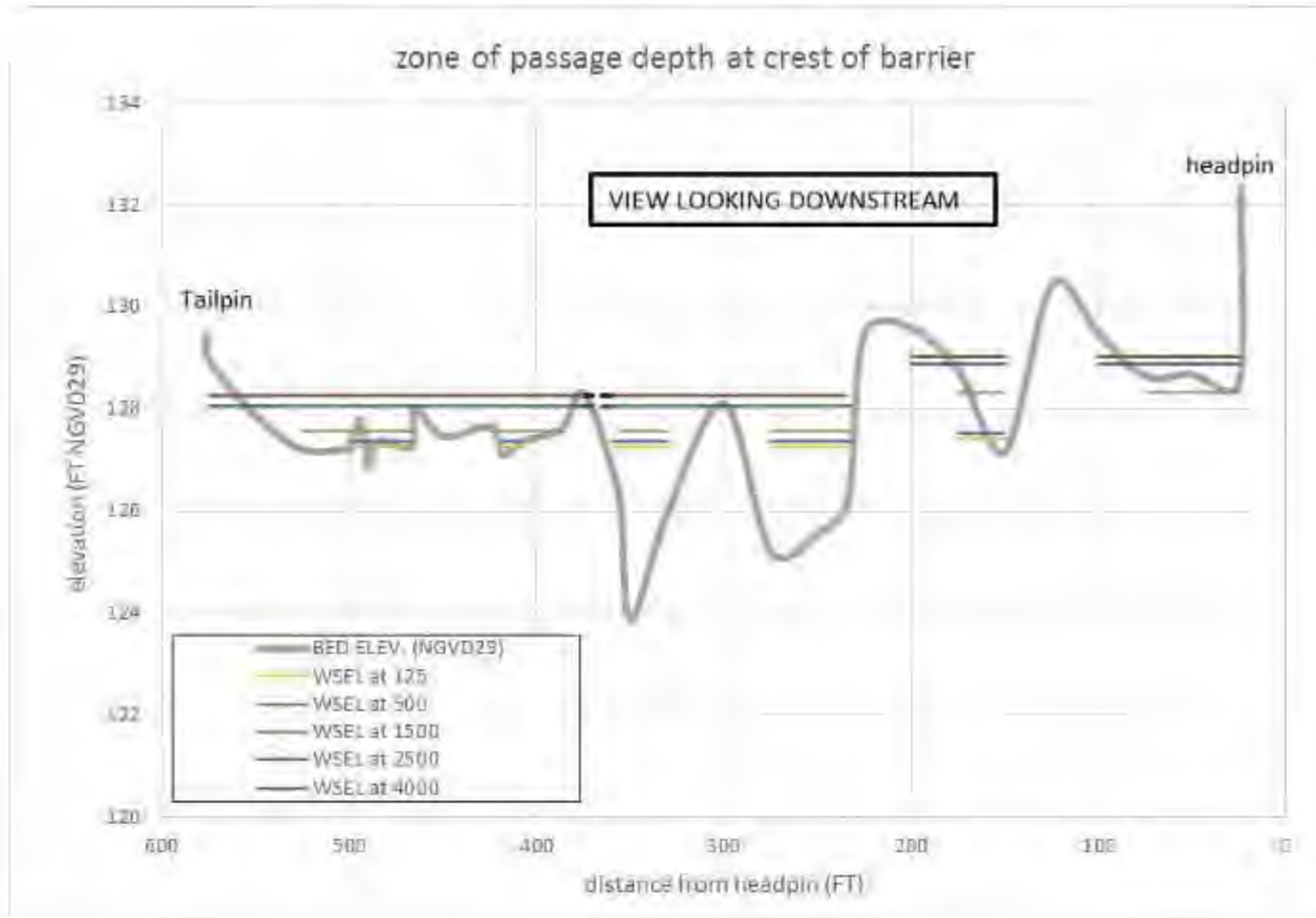
Figure 6.1.1.3-1: Left Channel Transect Elevation Survey in Upper Bypass Reach (Flow values relate to gate releases, not flow in channel)
