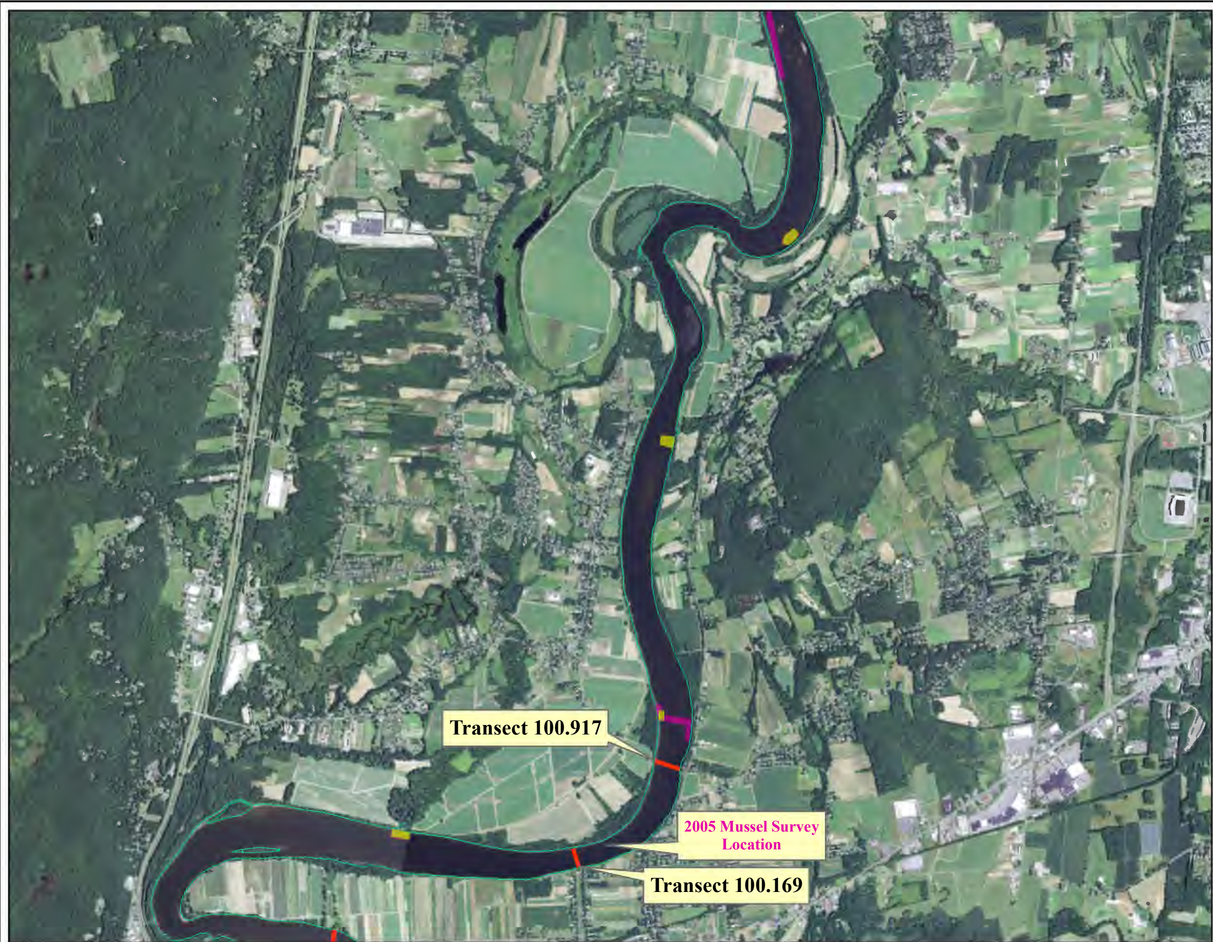
FIRSTLIGHT POWER RESOURCES IFIM Figure 5.3.5-1: Reach 5 HEC-RAS Transects Page 2 of 4
