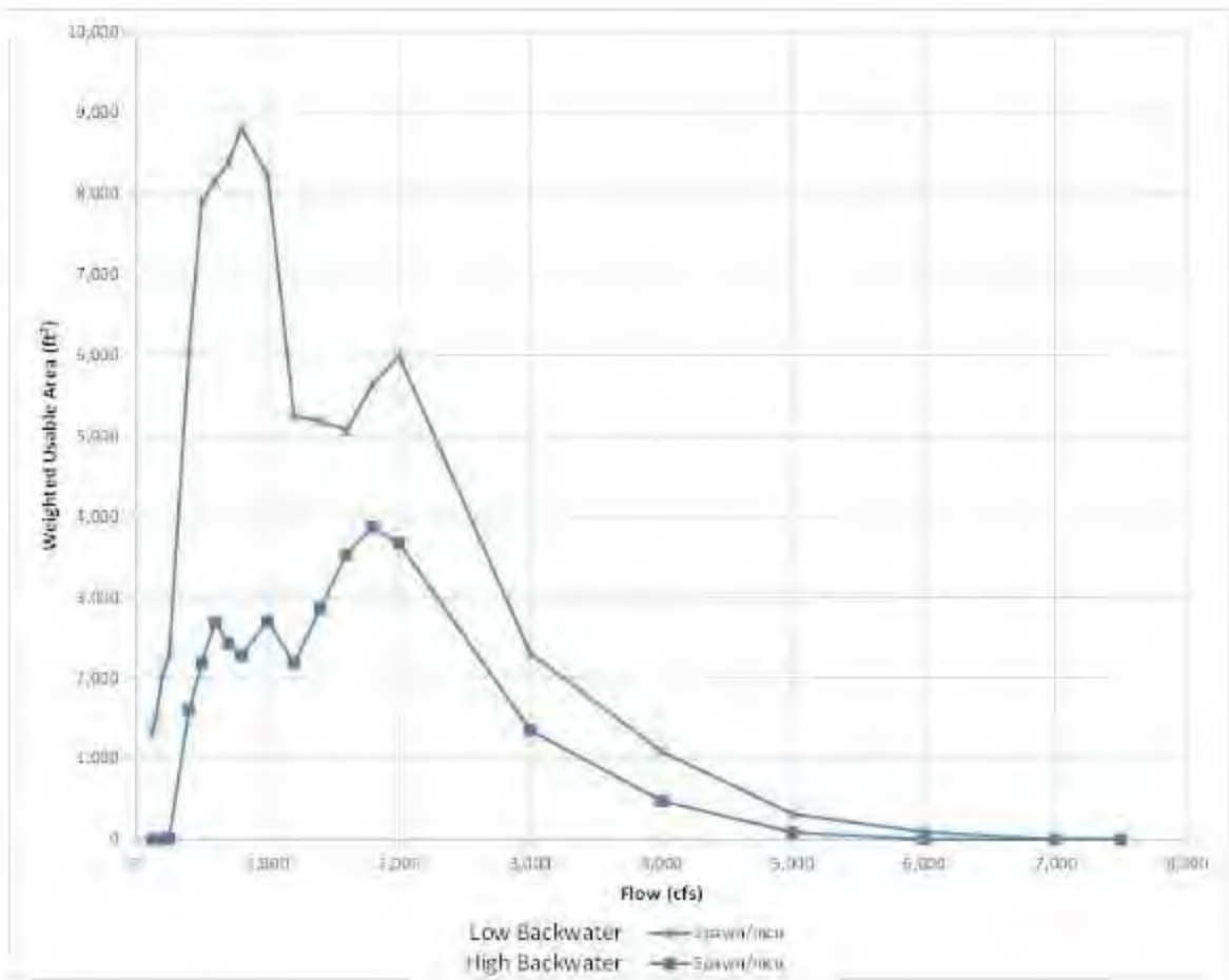
Figure C-8: Reach 1 (Transects 10 & 11) WUA curves for the spawning & incubation life stage of Sea Lamprey
