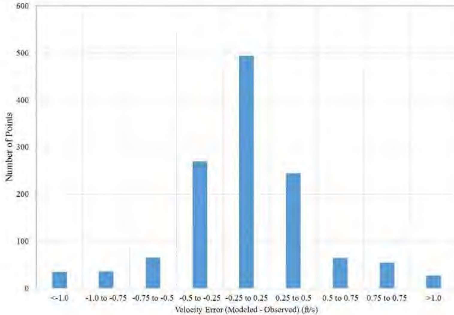
Figure 6.1.3-2: Velocity Error Distribution Reach 2B and 3
