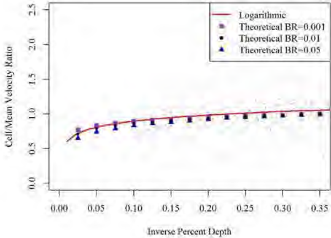
Figure 5.4.5-2: Comparison of Empirical Logarithmic Model with Theoretical Model Applying Different Bed Roughness Values
