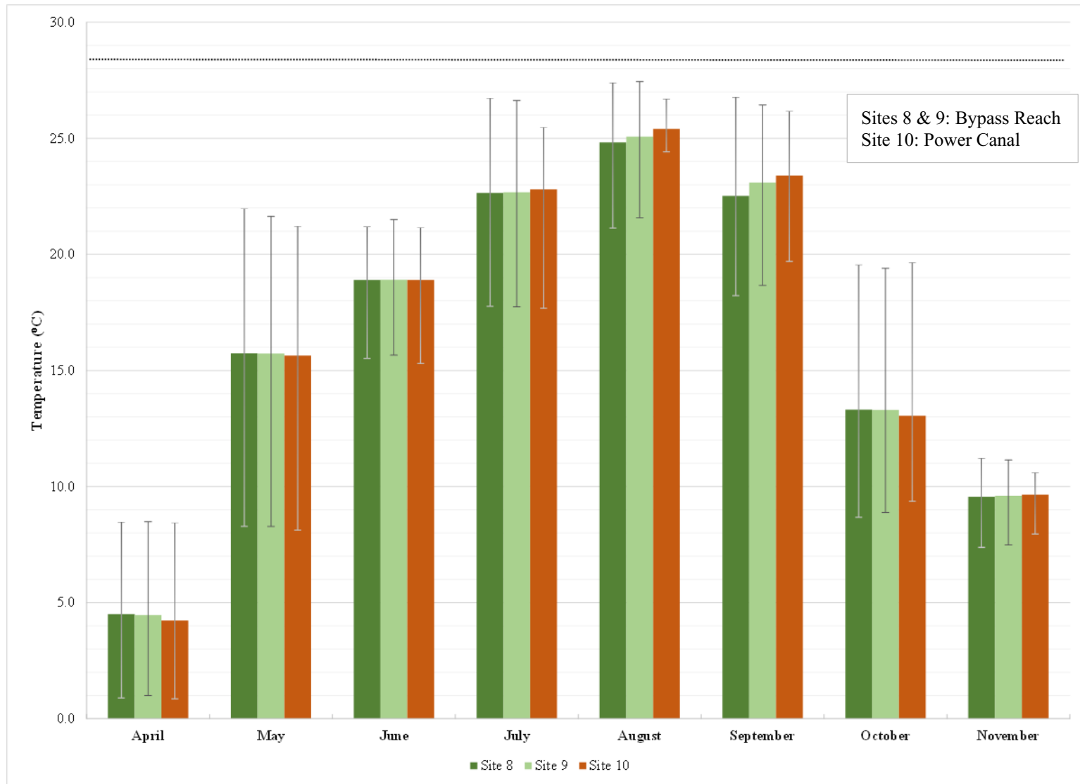
Figure 3.3.2-2: Monthly Average, Minimum and Maximum Temperatures for the Bypass Reach and Power Canal Locations
