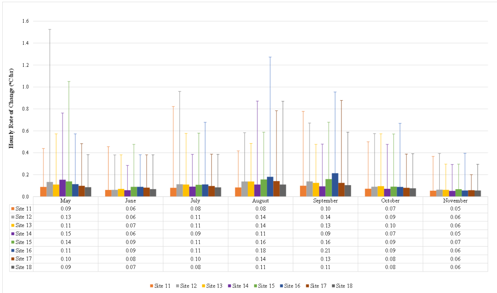
Figure 3.4.5-5: Monthly Average and Maximum Temperature Rate of Change (RoC)
