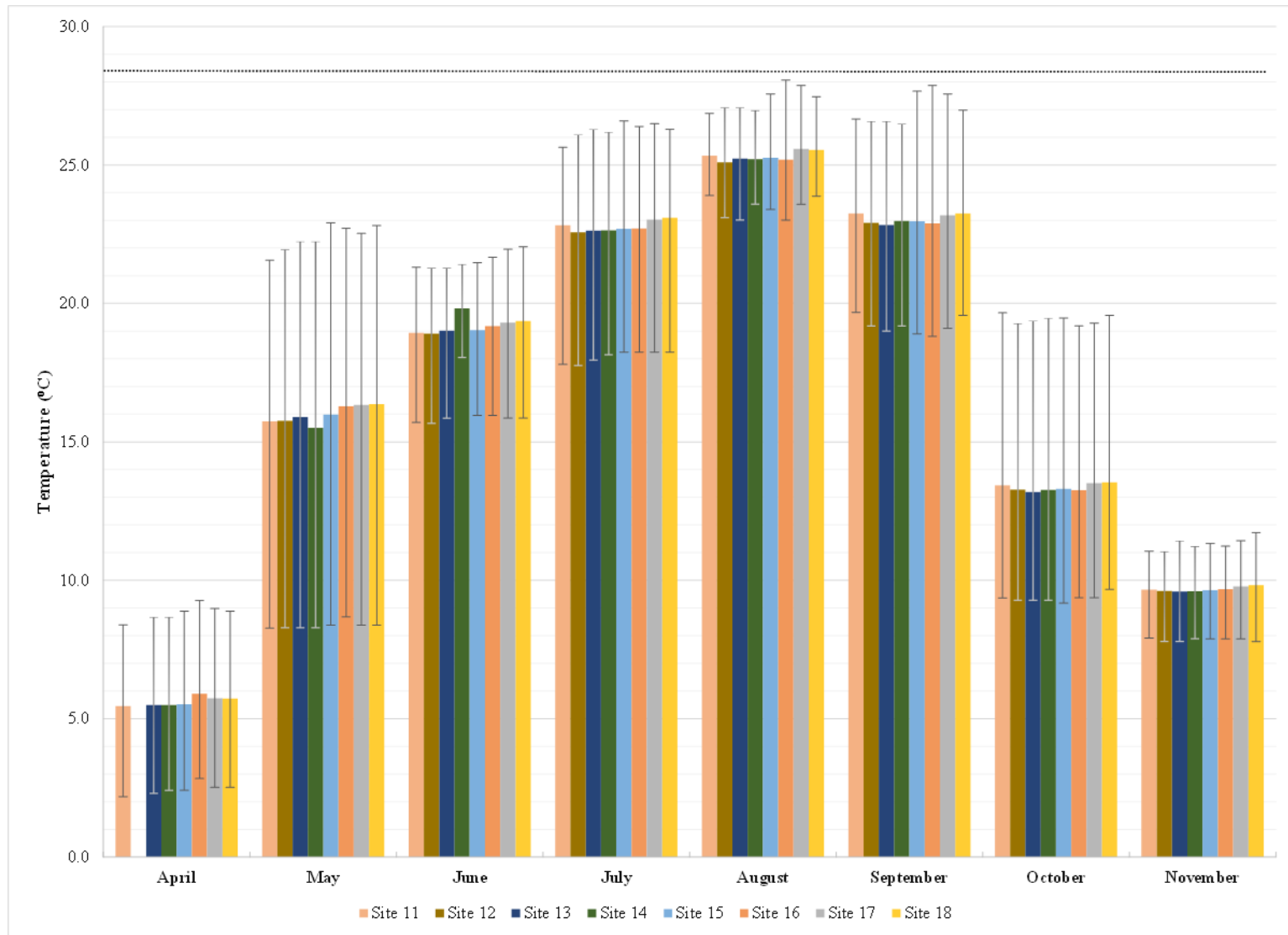
Figure 3.3.2-3: Monthly Average, Minimum and Maximum Temperatures for Locations below Cabot Station
