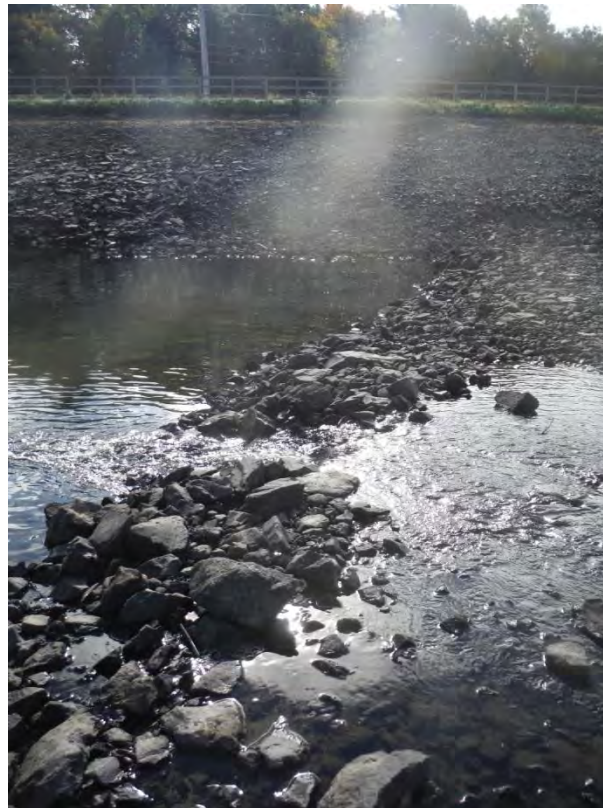
Photo 10. Riprap "weir" spanning canal bed in Zone 6. Note upstream direction of flow (Day 2).
