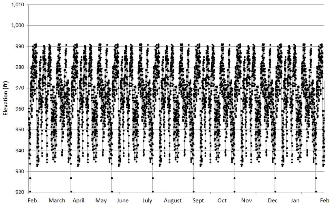
Figure 32. Case 3 Water Surface Elevation– 920 ft Minimum Reservoir Level
