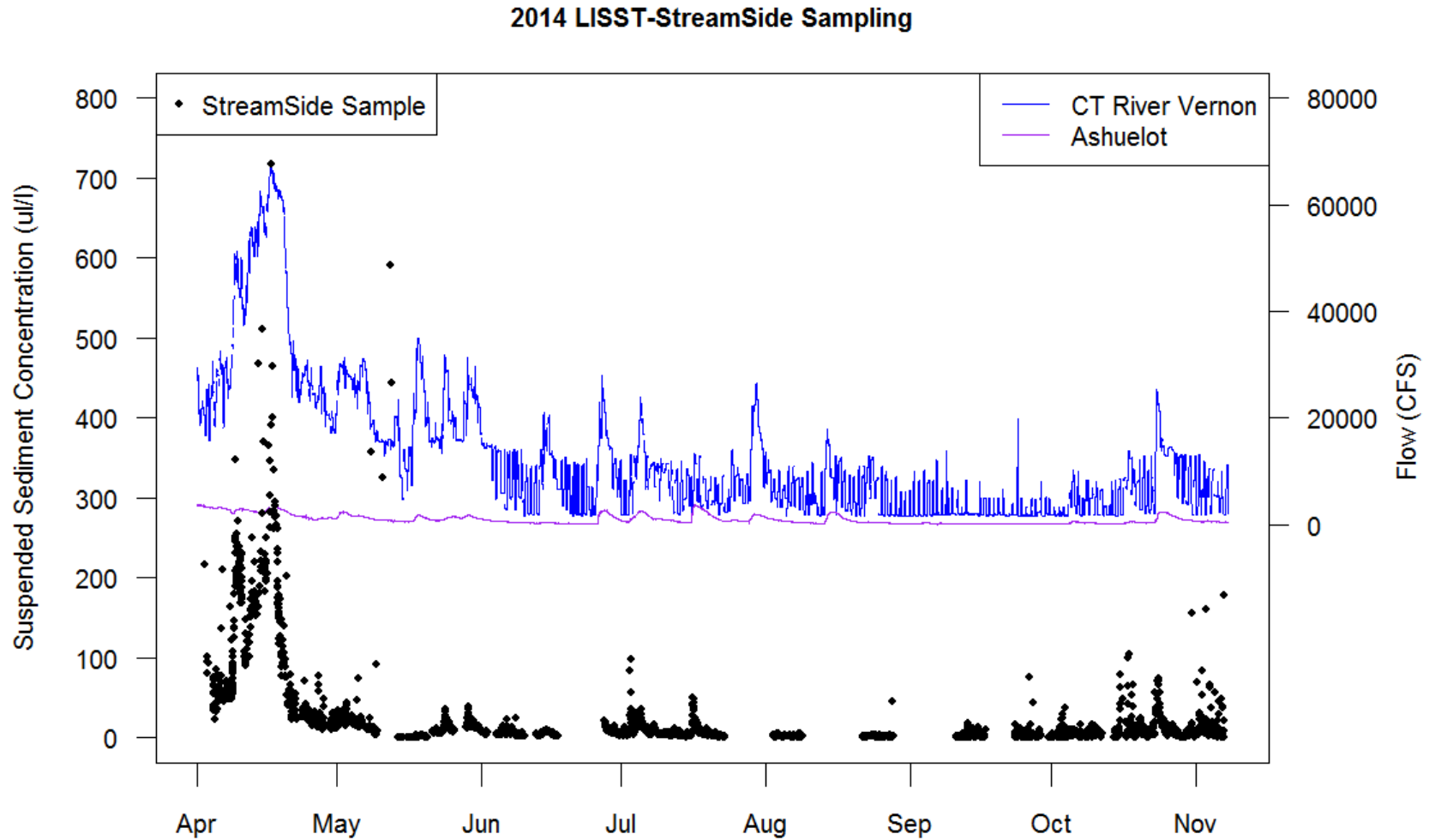
Figure 3.5: Provisional LISST StreamSide Suspended Sediment Concentration ( \mu\text{L} ) measurements collected in the vicinity of the Route 10 Bridge during 2014. 4 All data are provisional and subject to revision.
