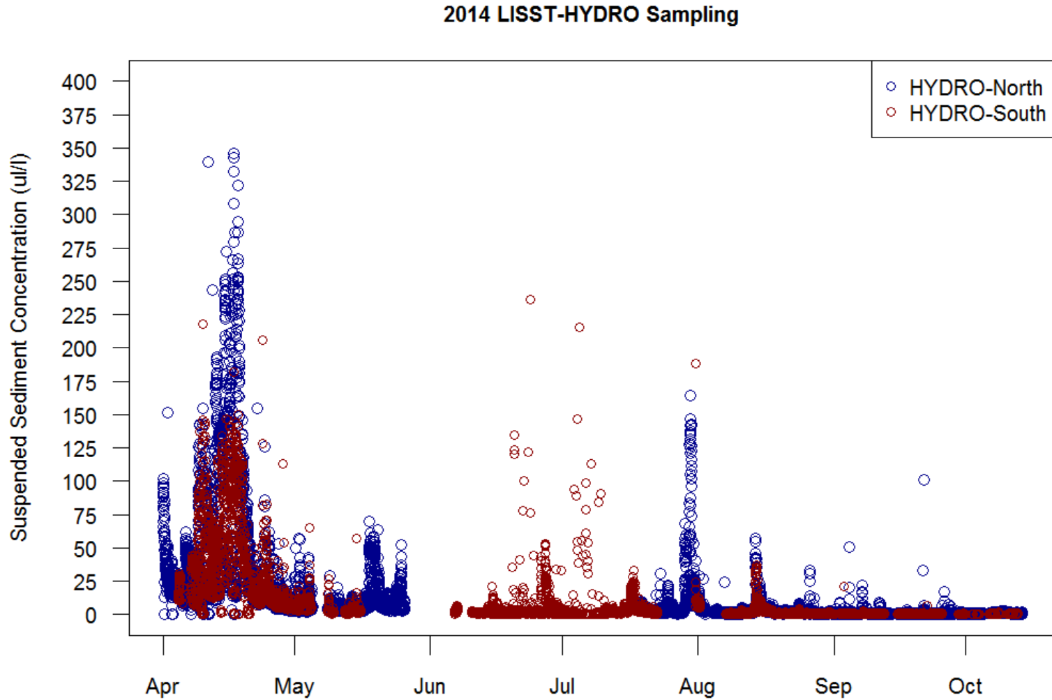
Figure 3.7: Provisional LISST HYDRO Suspended Sediment Concentration ( \mu\text{L} ) measurements collected in the Northfield Mountain Tailrace during 2014. 5 All data are provisional and subject to revision.
