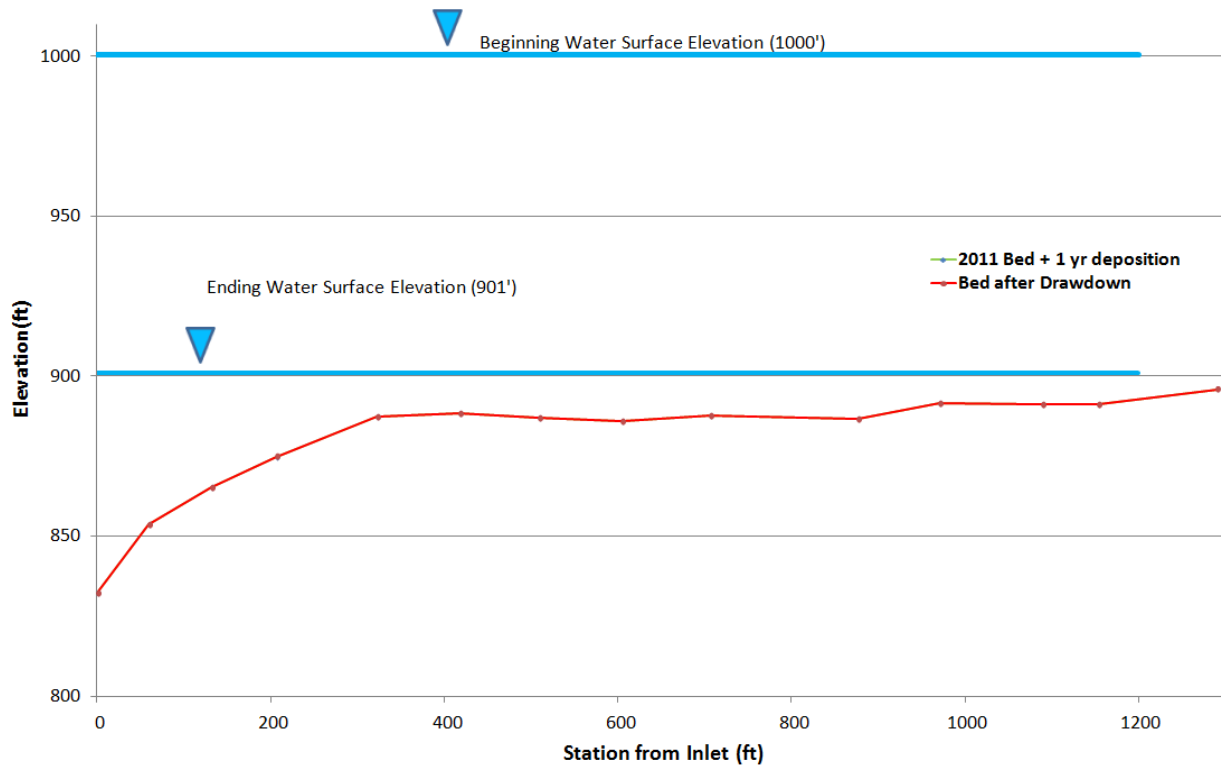
Figure 41. Sediment Mobilization Under Drawdown (Post 2010)
