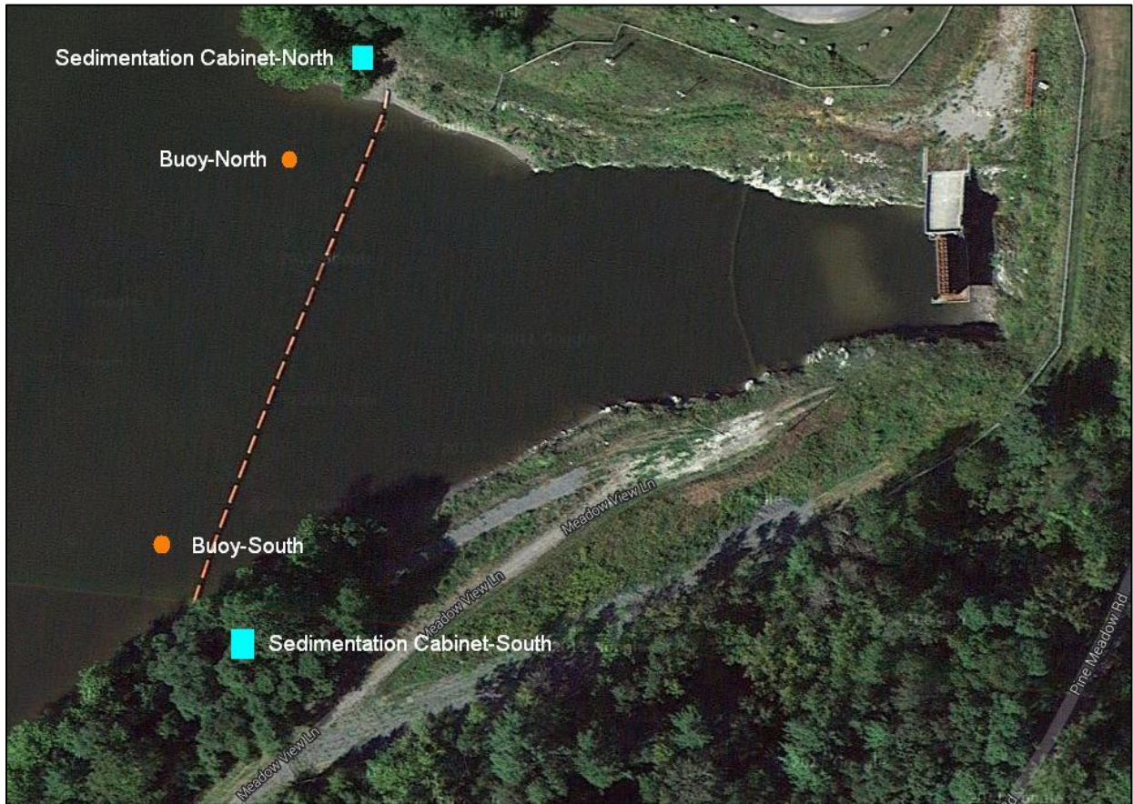
Figure 3.1: Aerial view of the Northfield Mountain Tailrace, showing LISST-HYDRO instrument locations.
