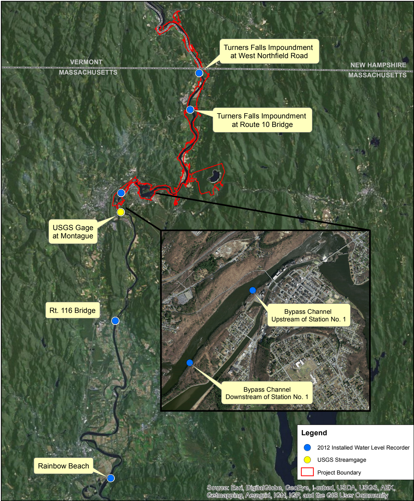
Figure 3.3.2-2 2012 Installed Water Level Recorder Locations
