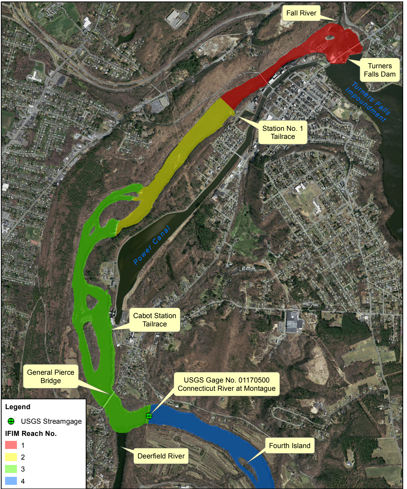
Figure 3.3.2-3: Proposed Instream Flow Study Reaches - Bypass Reach Inset
